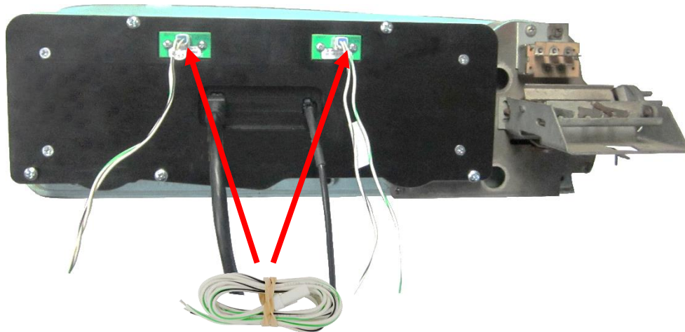
Indicator Harness
