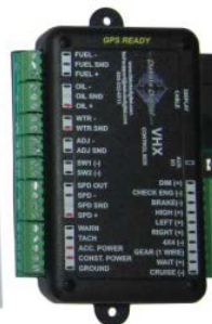
Control Box
