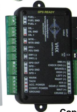
Control Box
