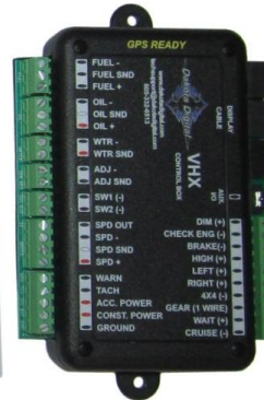
Control Box
