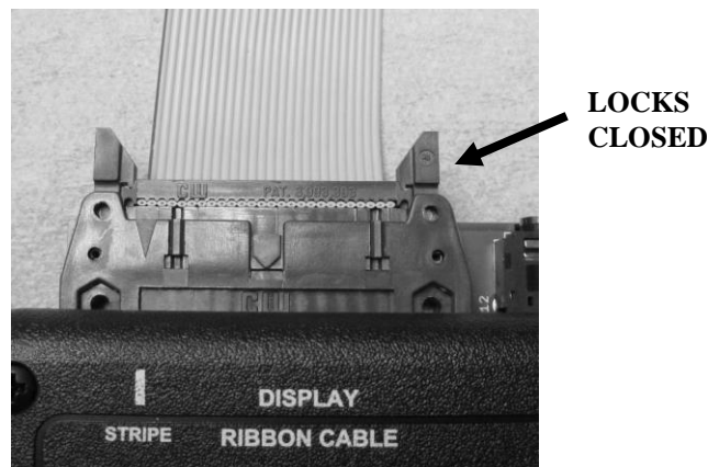
Ribbon cable connected
