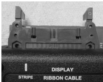
Locking tabs closed
