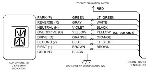
CONNECTION TO RON FRANCIS GEAR SHIFT INDICATOR SENDING UNIT.
