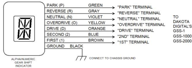
CONNECTION TO DAKOTA DIGITAL'S UNIVERSAL GEAR SHIFT SENDER (GSS-1, GSS-1000 or GSS-2000).
